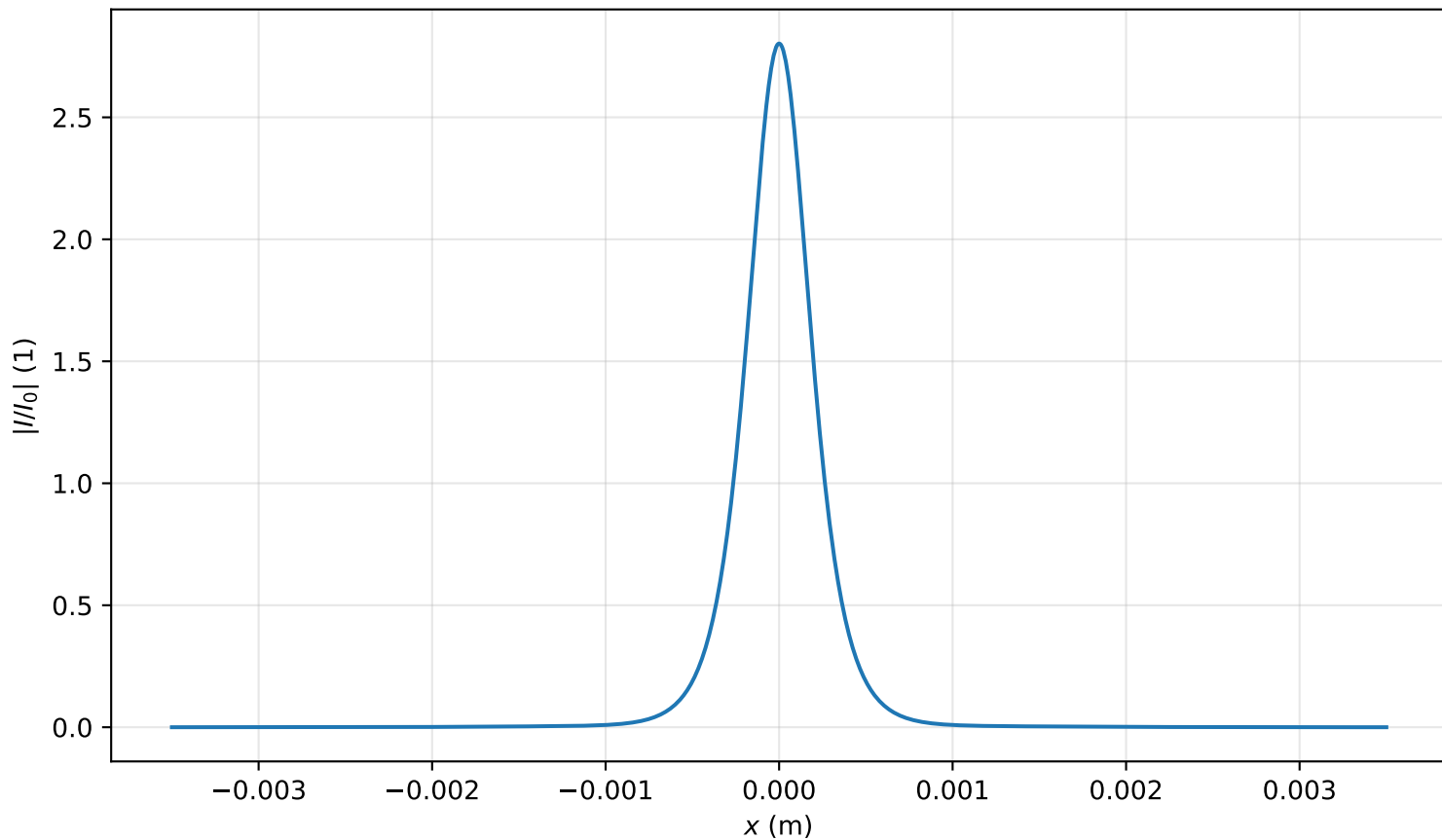
Intensity profile I(x, y = 0, z = 3.264m)/I_0 , P_{in}=1.0P_{cr} , artificial time
